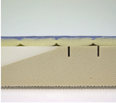
13 cm = 355 €/m 2
